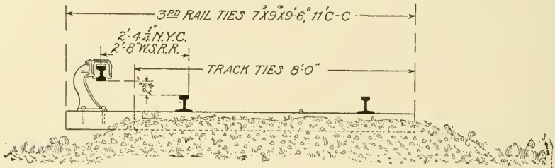
Fig. 203. Inverted Rail Insulator Mounted on Tie
